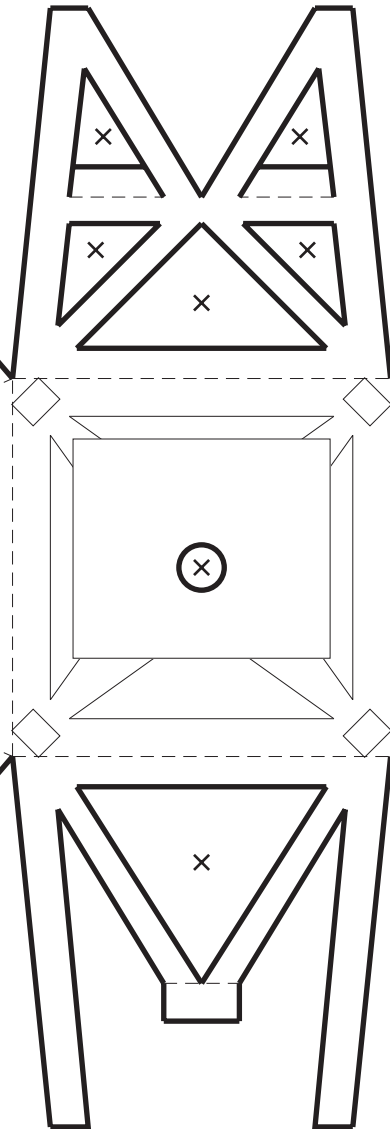
Sector gear
