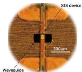
Superconducting device for ALMA's highest frequency receiver.
