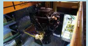
The wide-field multi-object spectrograph, Prime Focus Spectrograph (PFS), is mounted at the prime focus of the Subaru Telescope. It can simultaneously observe up to 2,394 objects across its 1.3 degree diameter field-of-view. (top) One of the spectrograph modules in the telescope dome. (bottom) The Prime Focus Instrument, together with the Wide Field Corrector, mounted at the prime focus of the telescope.
