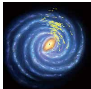
▲The position of 114 sources in the Galaxy measured by VERA, VLBA and EVN.
