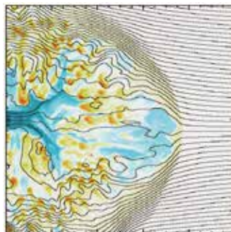
▲ A magnetohydrodynamics simulation of interactions between an astrophysical jet (blue) and interstellar clouds (orange). Black lines show magnetic field lines. The jet accelerates the dense interstellar clouds during the propagation of the jet. This simulation revealed that the magnetic field enhances the acceleration of the dense clouds by the magnetic tension force.
