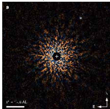
▲An image of a high-contrast space telescope with a coronagraph. Currently, Strategic Explorations of Exoplanets and Disks with Subaru Telescope (SEEDS) and IR planet hunting instrument development (IRD), TMT coronagraph (SEIT) development, WFIRST coronagraph (WACO) R&D are also ongoing.
