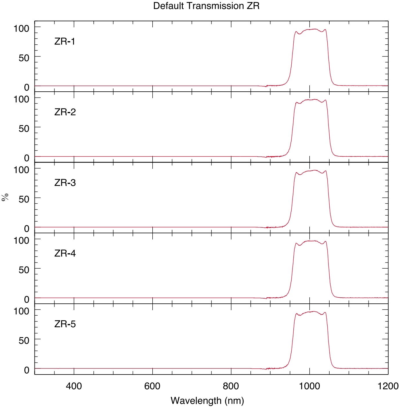
Figure 5: The default transmission curve of ZR.
