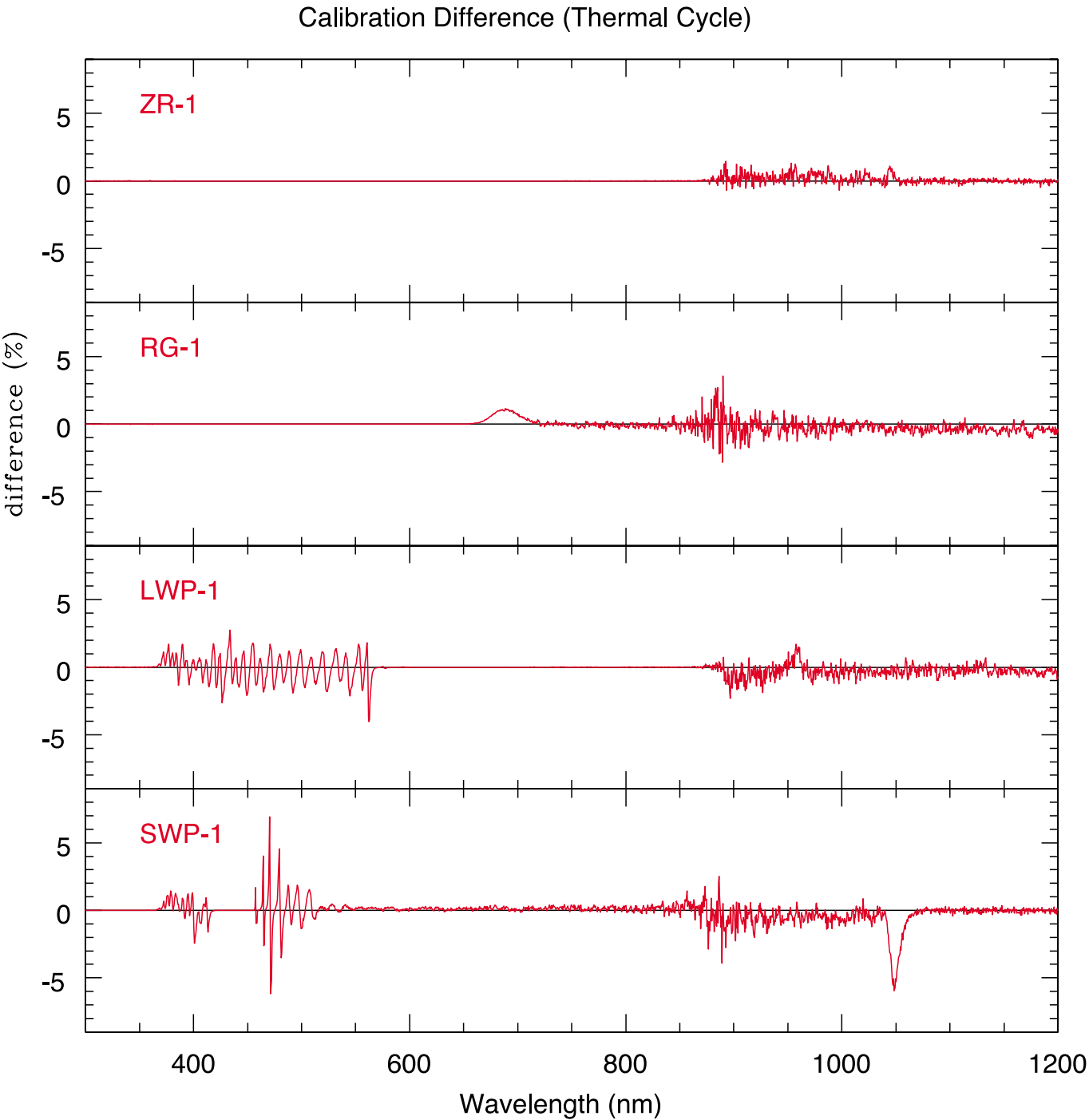
Figure 21: The difference obtained from the calibration measurement after the thermal cycle test.
