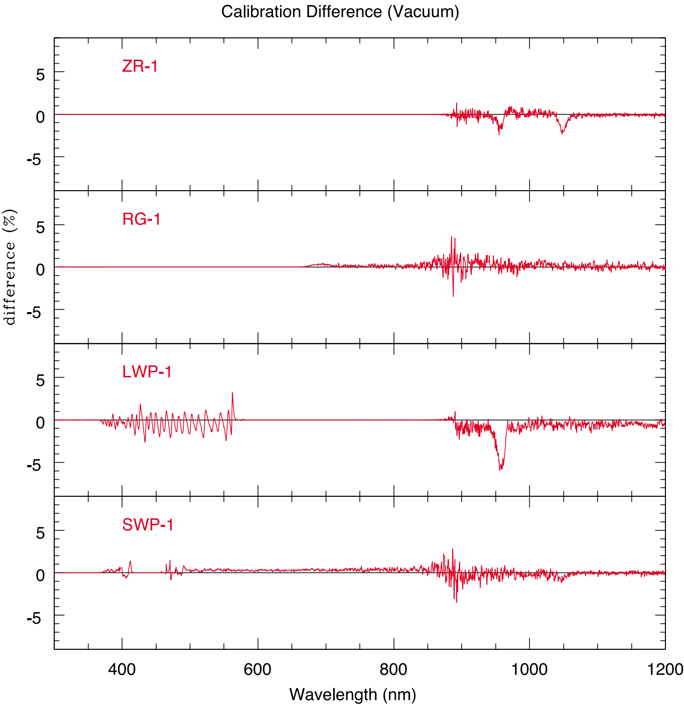
Figure 15: The difference obtained from the calibration measurement after the vacuum test.
