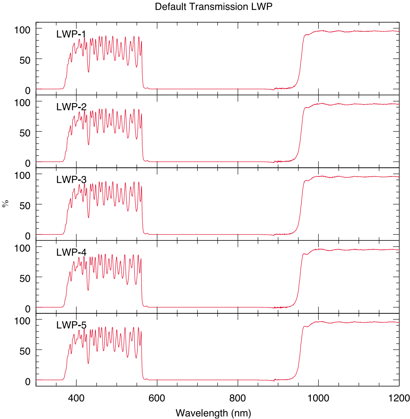
Figure 7: The default transmission curve of LWP.
