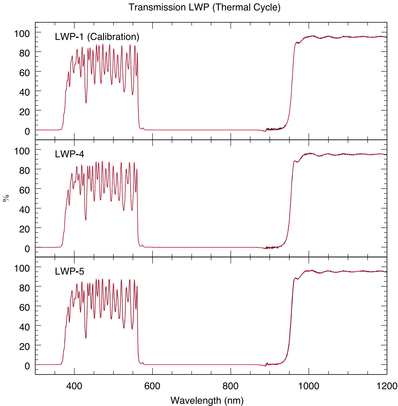
Figure 19: Transmission curves (red) of LWP after the thermal cycle test. The black curves are the default curves.
