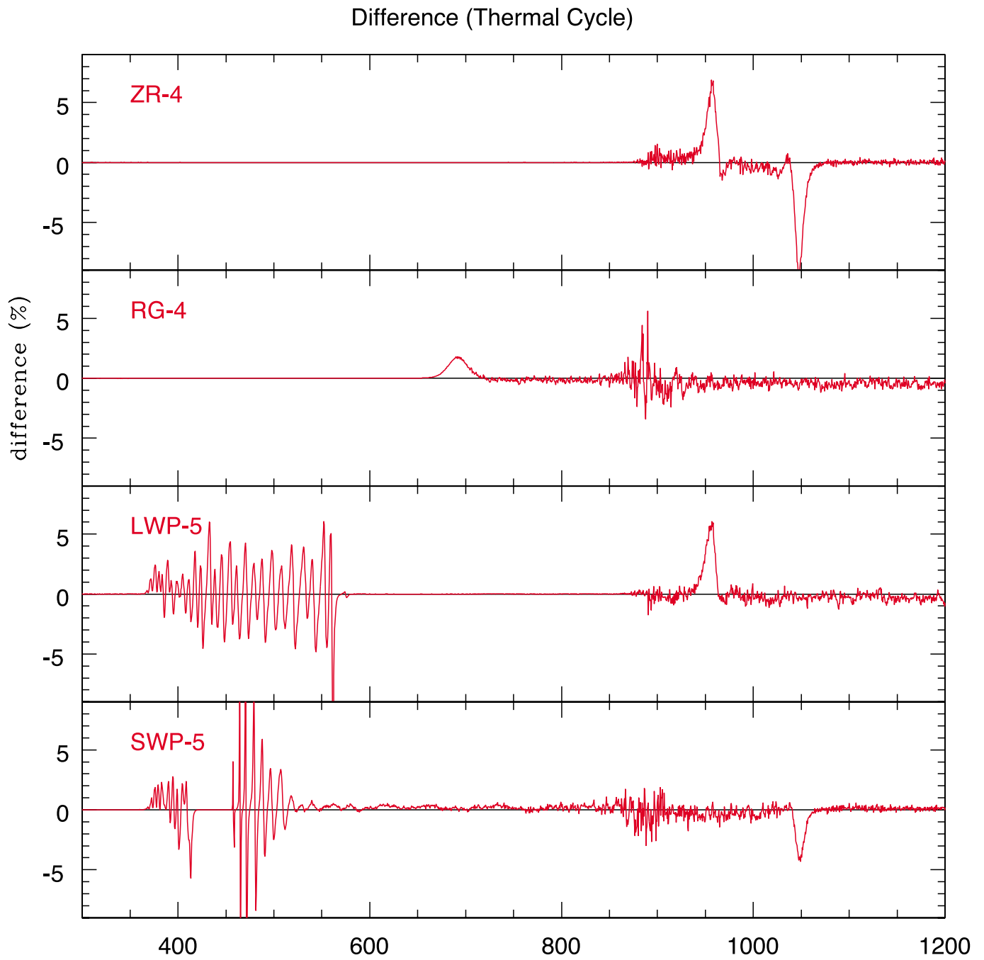
Figure 22: The largest difference between the default curve and the curve after the thermal cycle test.
