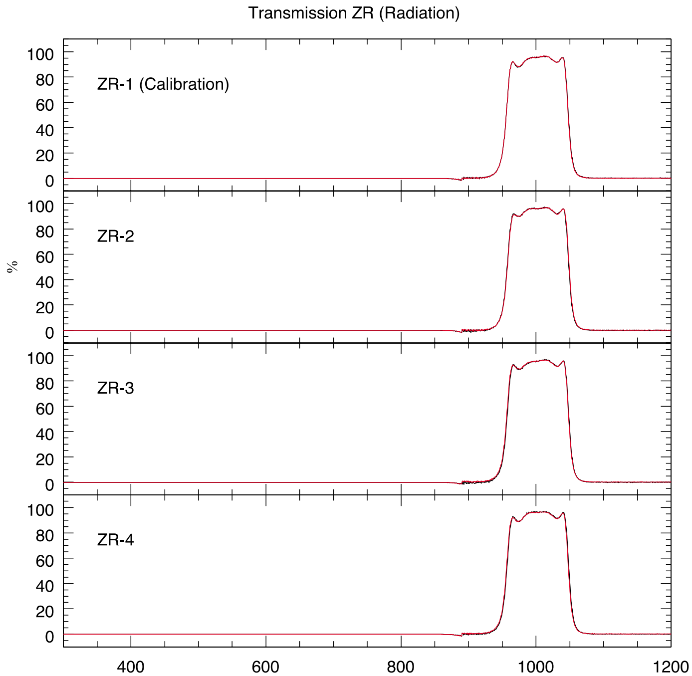
Figure 23: Transmission curves (red) of ZR after the radiation test. The black curves are the default curves.
