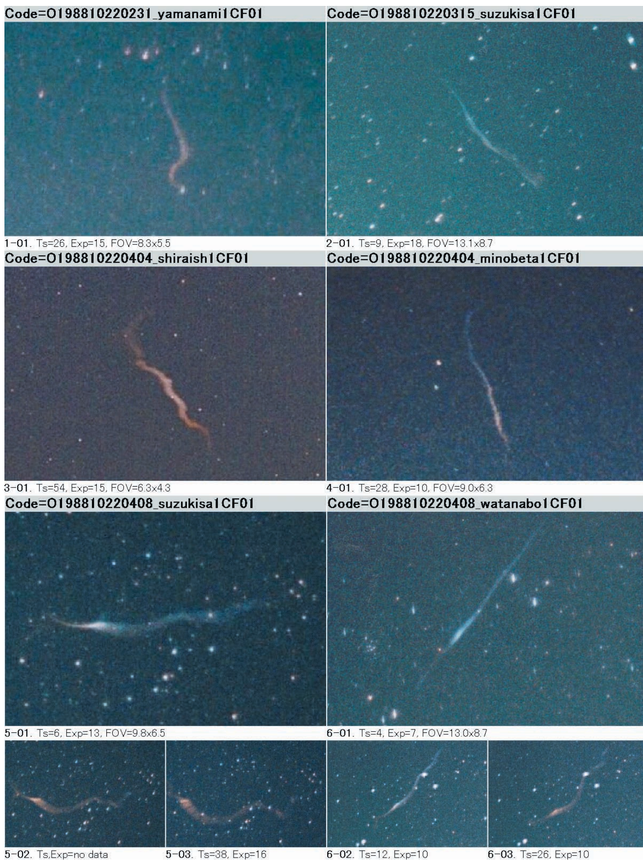
Fig. 4-1. Image sequences of the persistent train No. 1 to No. 6. Image sequences of No. 3 and 4 as well as No. 5 and No. 6 were simultaneously observed with each other.
