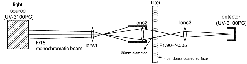
Fig. 1. Schematic figure of the F/1.9 beam generator.
