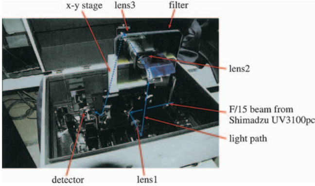
Fig. 2. A picture showing the F/1.9 beam generator and a filter put into Shimadzu UV3100pc spectro-photometer.
