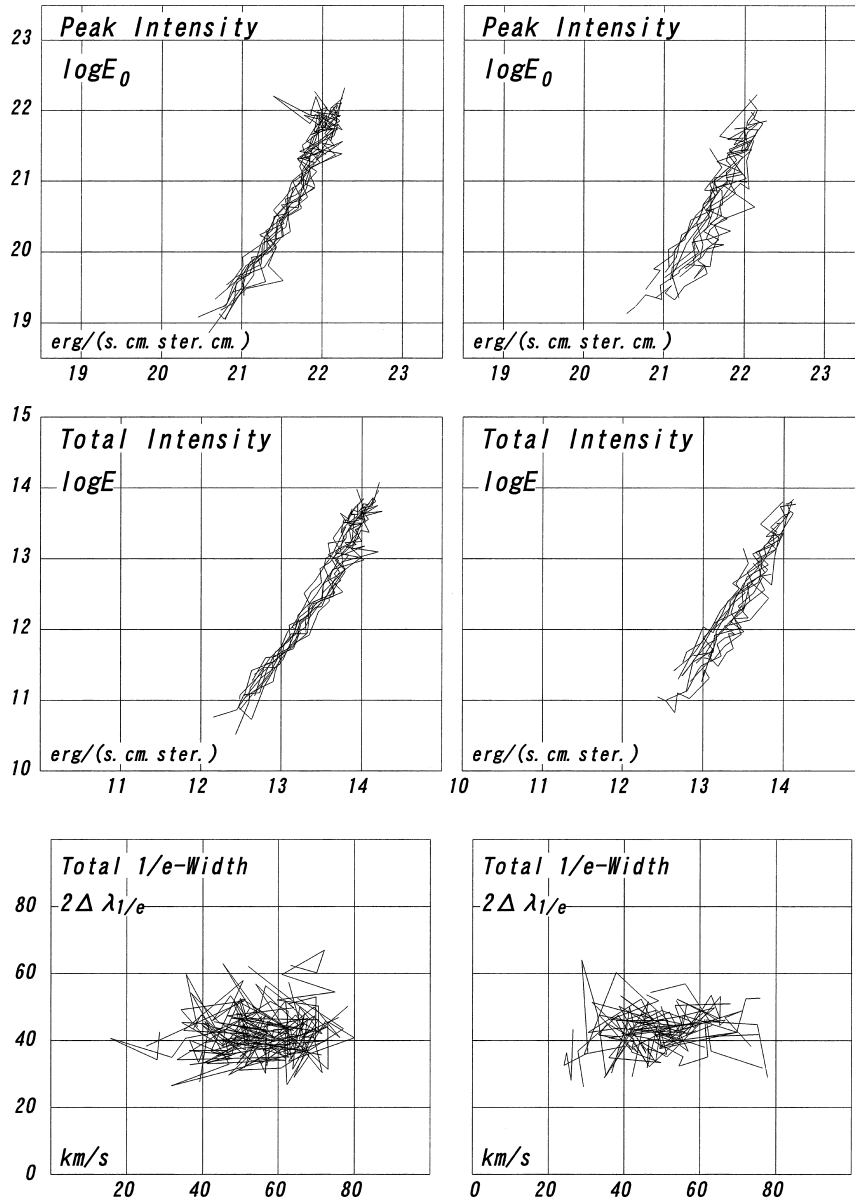
Fig. A2. Correlation between Ca II H (abscissa) and H \epsilon (ordinate) emissions from the 1958 eclipse data.
