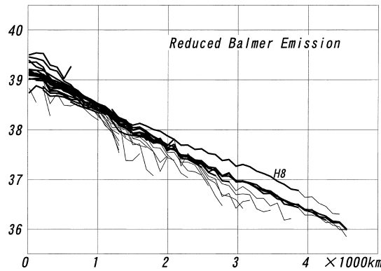
Fig. A3. Reduced Balmer line emissions to the integrated n_{\text{enp}} . H8 runs higher due to the blend with the He line. The part with the thin lines corresponds to the weaker intensity, \log E < 11.8 , and they run lower, probably due to a calibration problem.
