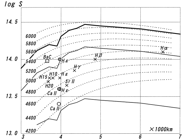
Fig. 12. Source functions of the emission lines. The open and gray circles are from the 1958 eclipse and for the less active and active regions, respectively. The crosses are from the 1962 eclipse. The square corresponds to the ionization temperature of the second level of hydrogen. The thick curve shows the photospheric brightness (Allen 1973). The thin curves are half and one tenth of the photospheric brightness. The dotted curves are brightnesses with the equivalent temperatures shown at their left ends.
