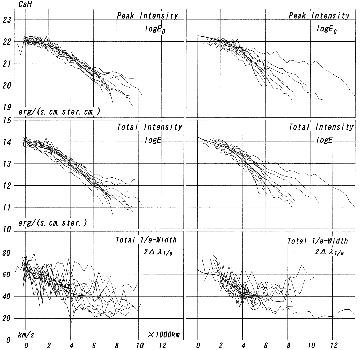
Fig. 4a. Fitting of the calculated curves (thick) to the observed Ca II H eclipse curves (thin).
