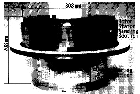
Fig. 1. A newly developed resolver with an accuracy of 30 mas rms.
