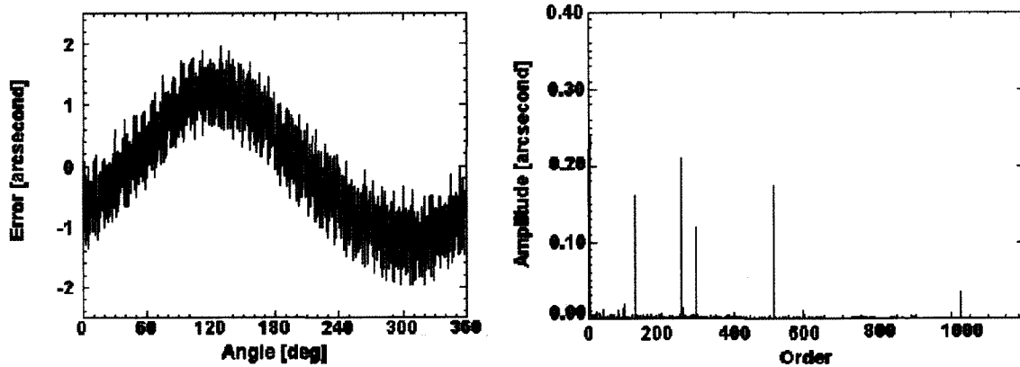
Fig. 3. Measurement of raw readout of the azimuth encoder (left) and its Fourier components (right).
