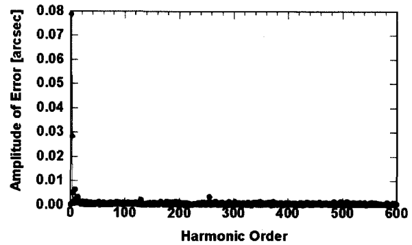
Fig. 5. Fourier components of error due to shaft radial misalignment of 0.10 mm.
