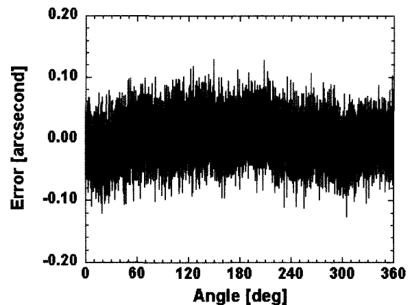
Fig. 4. Angle errors of readouts after PROM compensation.
