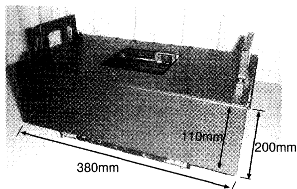
Fig. 3. b: The photograph of the exchanger attached a enclosure. The filter exchanger is mounted on the dewar in this style.
