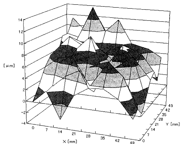
Fig. 2. c: The change of the CCD surface under the cooled condition from that under the room temperature. The peak-to-valley was within 16\mu\text{m} .
