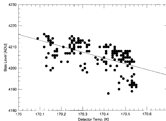
Fig. 7. The bias level against the detector temperature. The bias levels were measured at the overscan regions and had a loose anti-correlation with the detector temperature. The solid line shows the regression line and its slope was -28\text{ADU/K} .
