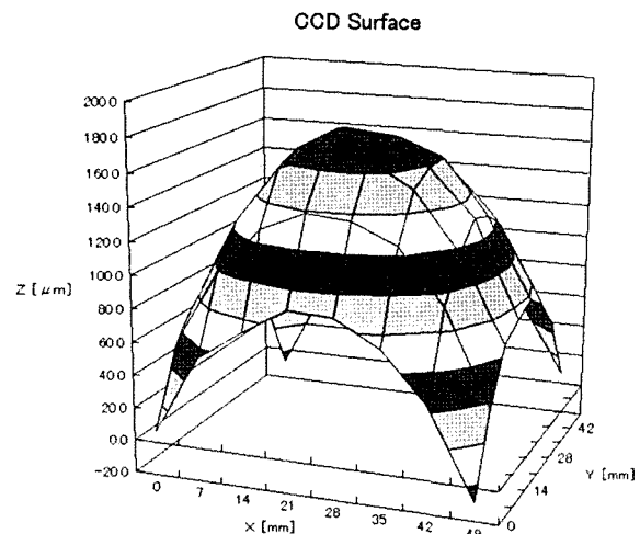
Fig. 2. a: The bird's-eye map of the CCD surface under the cooled ( -100^\circ\text{C} ) condition.
