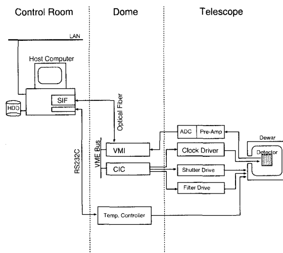
Fig. 4. The schematic view of our data acquisition system. The SBus interface (SIF), VME-memory interface (VMI), and CCD and instrument controller (CIC) constitute MESSIA. The clock driver, pre-amp, and ADC board, whose designs largely depend on the detector characteristics, were designed by ourselves. The camera is controlled by a workstation, Fujitsu S-4/5.
