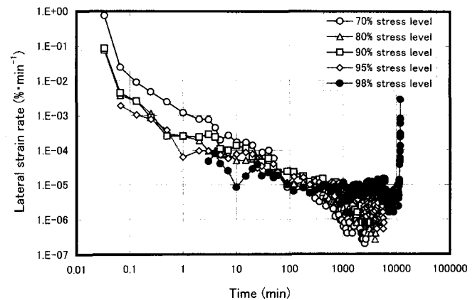
Fig. 7(b). Relationship between lateral strain rate and time.
