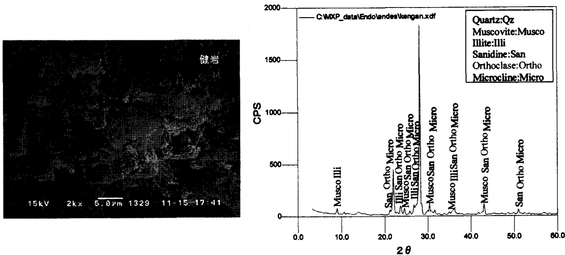
Fig. 2(a). SEM photograph and result by the X-ray diffractometer on intact rock sampled at the international road.
