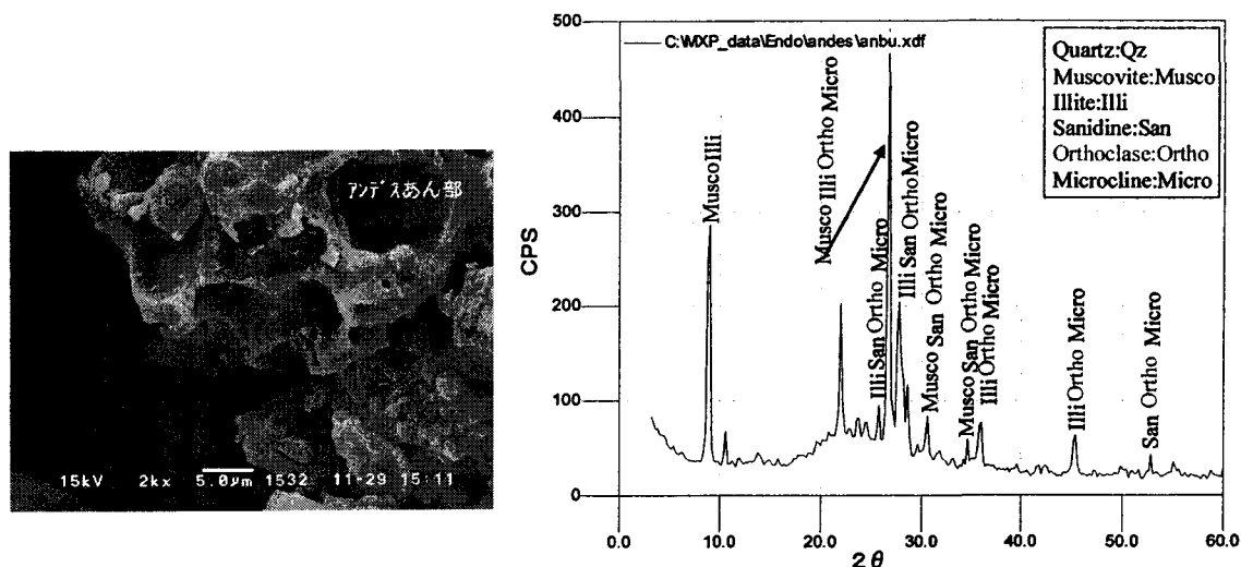
Fig. 2(g). SEM photograph and result by the X-ray diffractometer on sand sampled at No. 5 saddle site.
