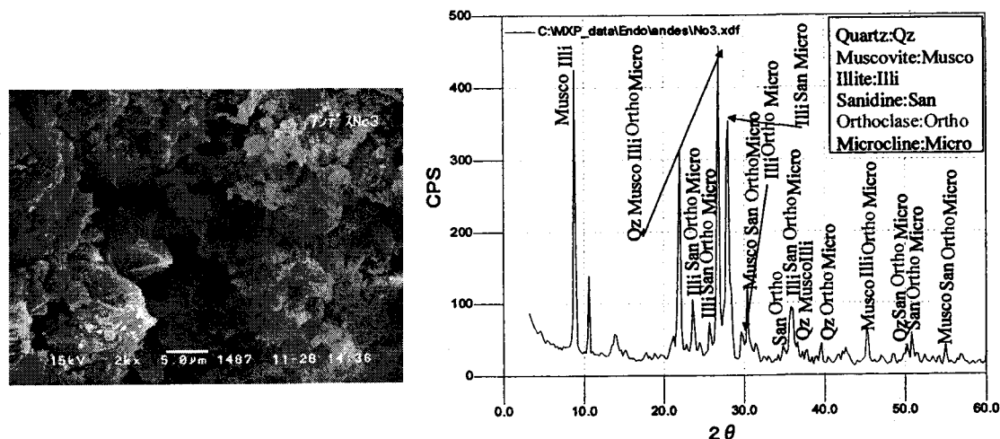
Fig. 2(d). SEM photograph and result by the X-ray diffractometer on pebble sampled at No. 3 site.
