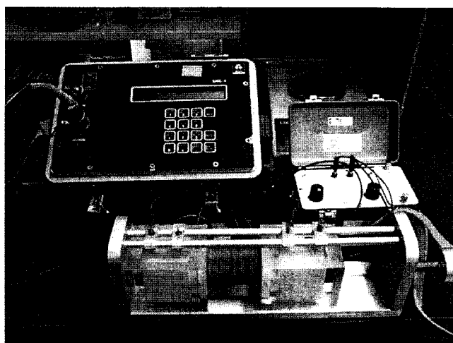
Photo 1. Overall view of the device for measuring the rock resistivity.
