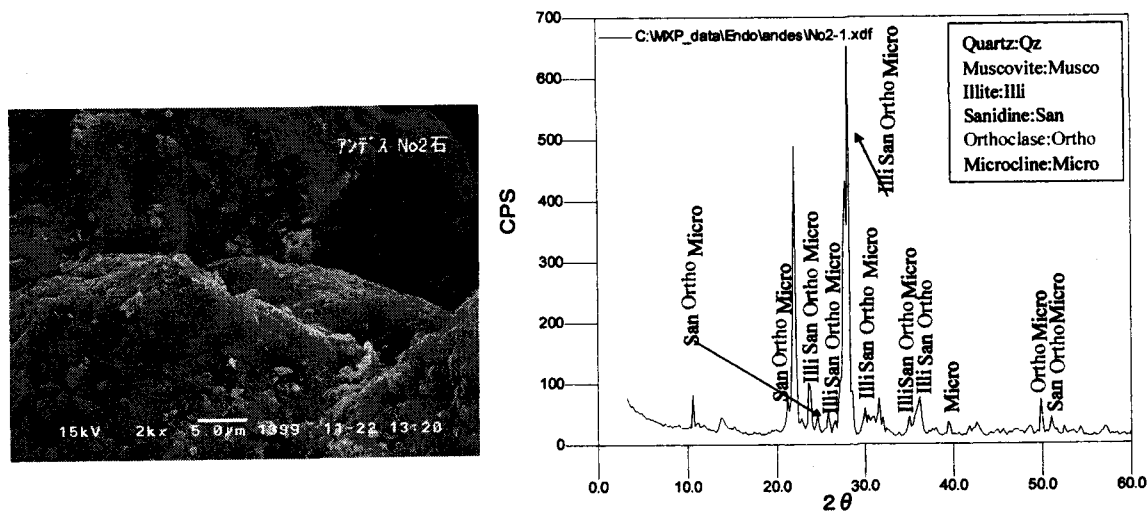
Fig. 2(b). SEM photograph and result by the X-ray diffractometer on pebble samples at No. 2 site.
