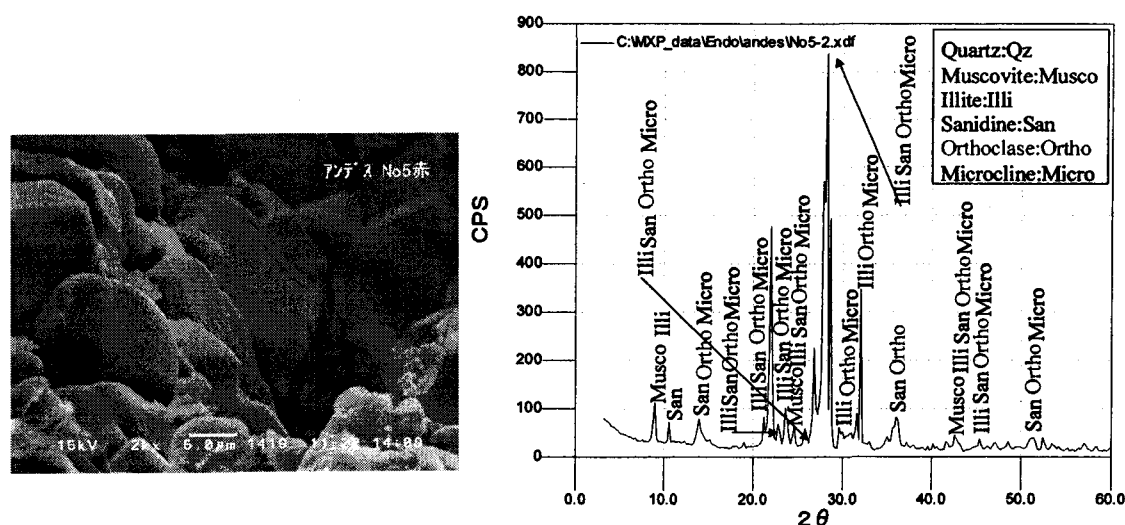
Fig. 2(f). SEM photograph and result by the X-ray diffractometer on red pebble sampled at No. 5 site.
