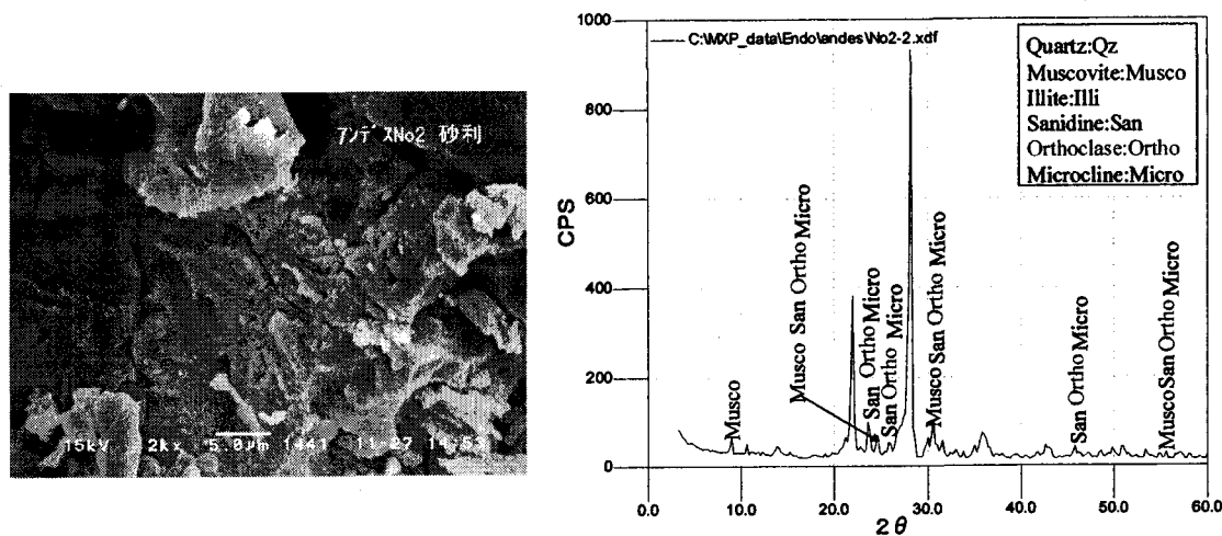
Fig. 2(c). SEM photograph and result by the X-ray diffractometer on sand sampled at No. 2 site.
