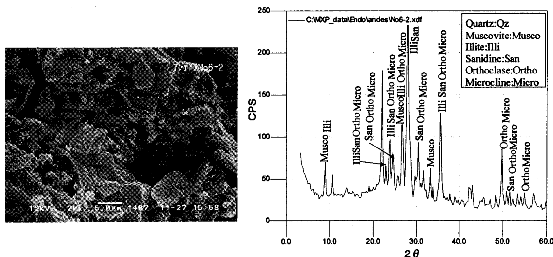
Fig. 2(h). SEM photograph and result by the X-ray diffractometer on pebble sampled at No. 6 site.
