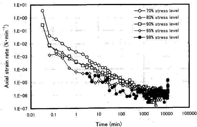
Fig. 7(a). Relationship between axial strain rate and time.
