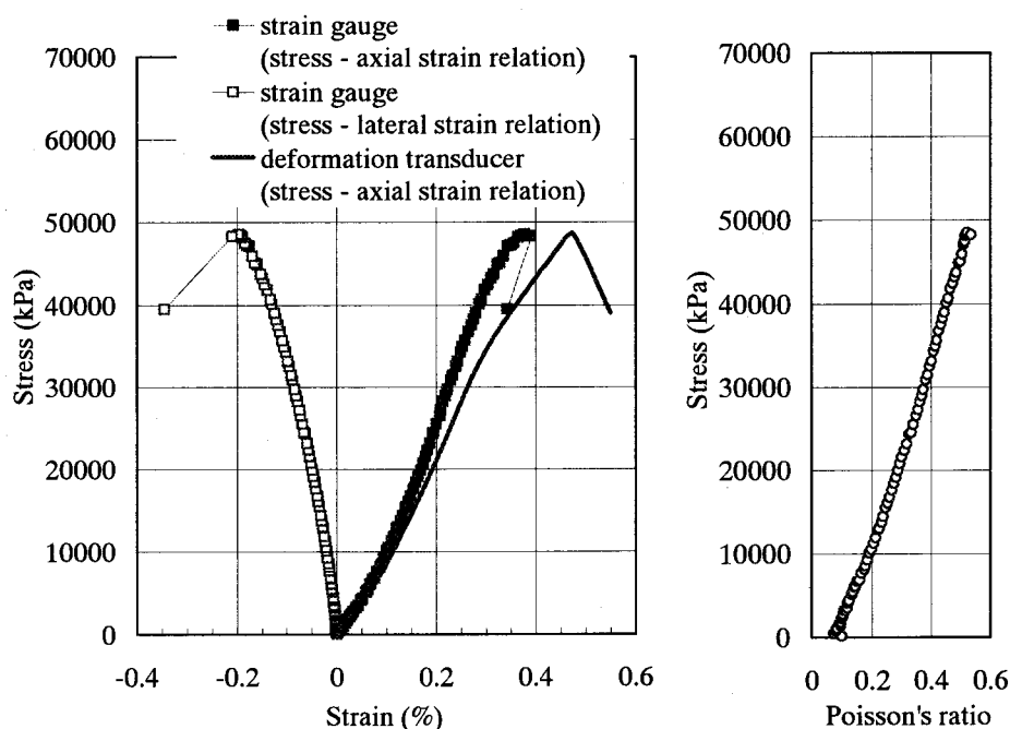
Fig. 6. Stress-axial strain relationship, the stress-horizontal strain relationship and the stress-Poisson's ratio relationship.
