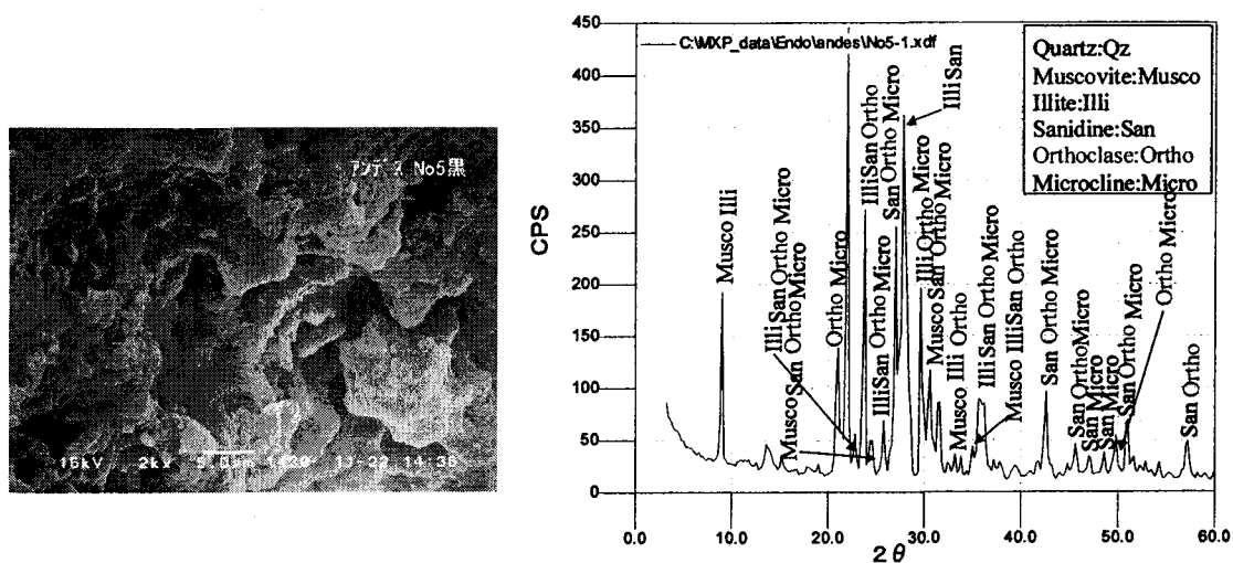
Fig. 2(e). SEM photograph and result by the X-ray diffractometer on black pebble sampled at No. 5 site.
