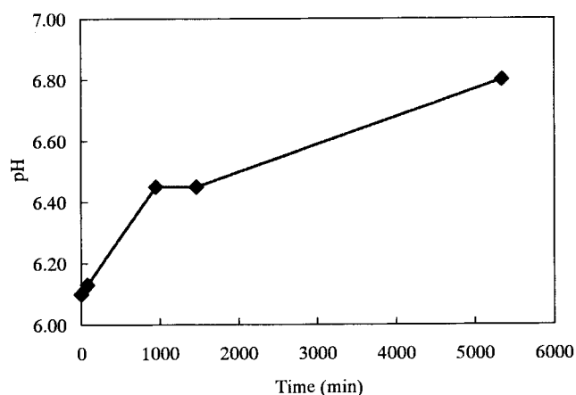
Fig. 3. Relationship between pH value and the time on intact rock sampled from No. 2 site.
