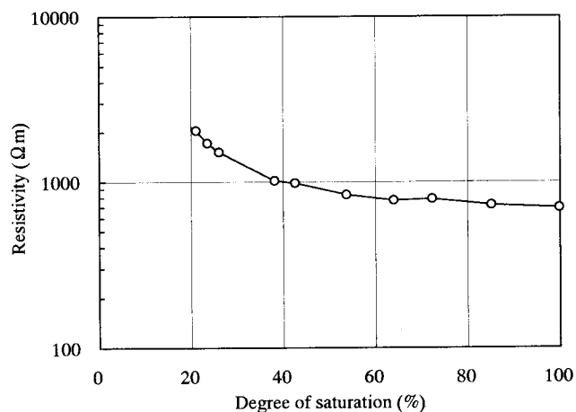
Fig. 5. Variation of the resistivity of the intact rock with respect to degree of saturation.
