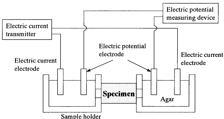
Fig. 4. Layout of the devices for measuring the rock resistivity.
