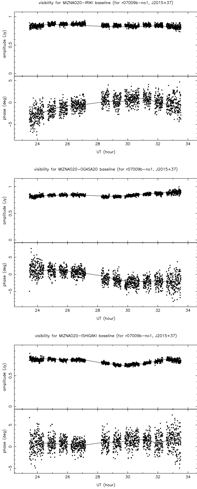
Fig. 3. (a: Top): The model (curve) and observed (dot) visibilities of J2015+3710 for the Mizusawa-Iraki baseline. The model visibilities are obtained from the CLEAN components of the self-calibration map. The observed visibilities are corrected for the station-based gain solutions obtained with the self-calibration. The upper panel shows the visibility amplitudes, and the lower panel shows the phases, respectively. (b: Middle): The same to figure 3a but for Mizusawa-Ogasawara baseline. (c: Bottom): The same to figure 3a but for Mizusawa-Ishigaki-jima baseline.
