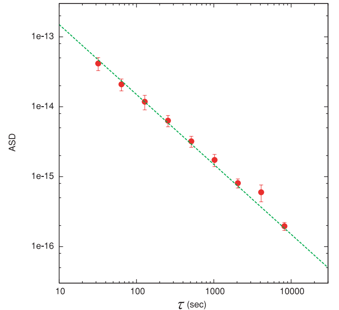
Fig. 7. Allan Standard Deviation (ASD) of the phase residuals obtained by using the data between UT 24.5 to 32.4 in figure 6. Here the ASD is obtained for each baseline and averaged over the six baselines. The error bars show the scatter of the ASD among the six baselines of VERA. The green line shows the behavior of the white-phase noise, characterized as \sigma_y \propto \tau^{-1} .
