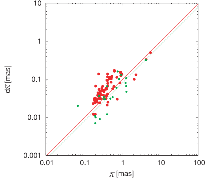
Fig. 8. Parallax amplitudes \pi versus parallax errors \sigma_\pi in VERA's results. Red spots are the results obtained by using one spot data, and green spots are those by combined fit to multiple maser spots. Regression lines (in the form of \sigma_\pi = a\pi ) for red and green spots are also shown.
