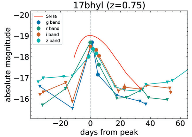
Figure 2: The multi-band and absolute-magnitude light curves of HSC17bhyl. The red line represent the i -band light curve of SN Ia generated by the sncosmo package.
