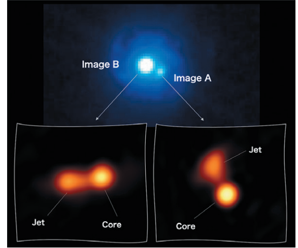
Figure 1: (Top) HST image of B0218+357 (credit: NASA/ESA and the Hubble Legacy Archive). (Bottom) KaVA 7mm images of lensed image A and B.
