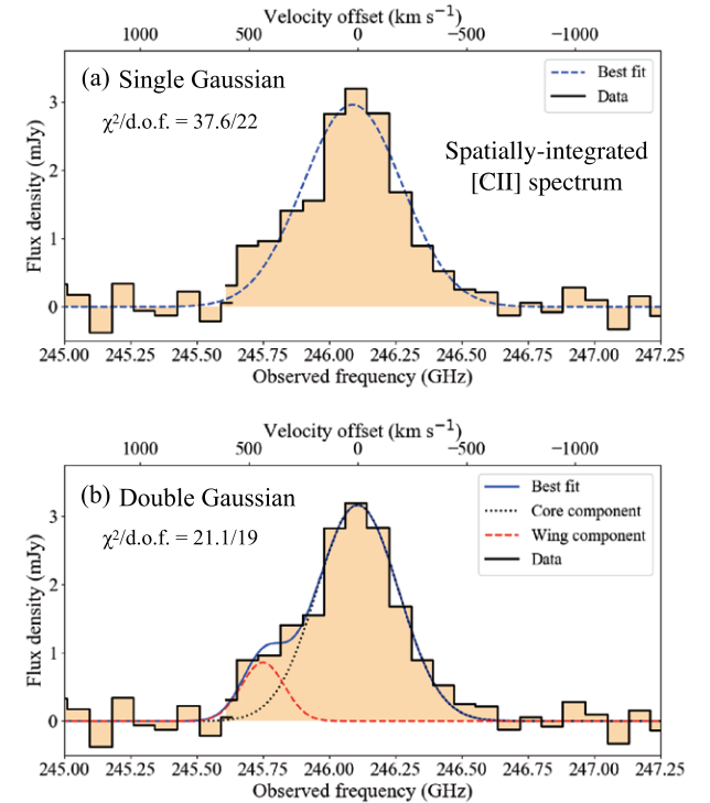
Figure 2: Spatially-integrated [CII] spectrum of J1205–0000. The observed spectrum cannot be well-fitted by a single Gaussian (top). We need to use at least a double Gaussian profile (bottom), which manifests the existence of multiple component in this system spectroscopically.
