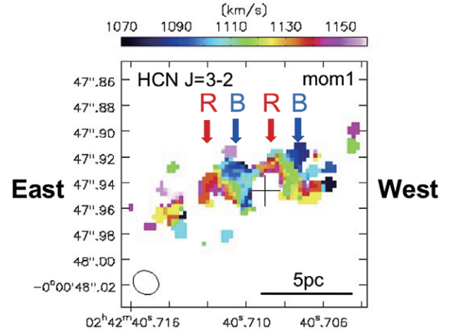
Figure 1: Intensity-weighted mean velocity (moment 1) map of HCN J = 3-2 emission line taken with ALMA 0.02'' ( \sim 1 pc) resolution observations. In the western torus, inner part is redshifted and outer part is blueshifted. In the eastern torus, inner part is blueshifted and outer part is redshifted. B and R means blueshift and redshift, respectively. Namely, the presence of counter-rotating dense molecular gas components was revealed in the torus [2]. SMBH position is shown as +.
