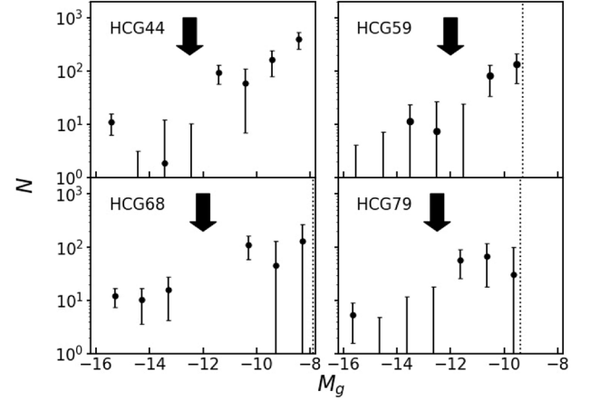
Figure 1: g -band LFs for individual groups of HCG44, HCG59, HCG68, and HCG79. The vertical dotted line indicates the 90 % completeness limit for each HCG. The arrows show the locations of the dip around M_g \sim -12 .
