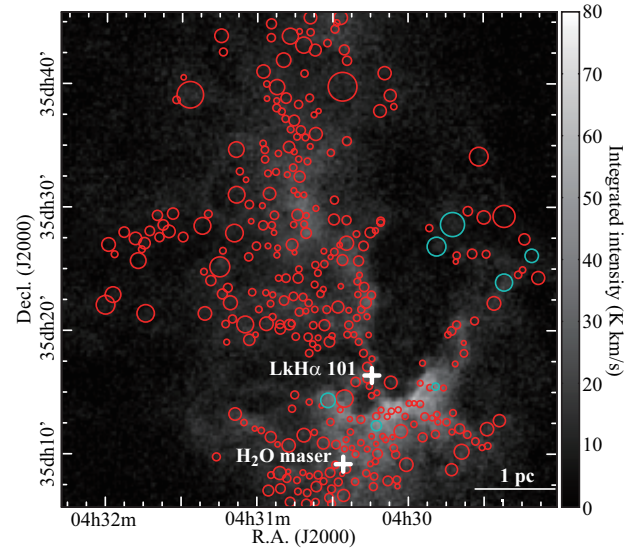
Figure 2: Integrated intensity map of the 13 CO( J = 1-0 ) emission line towards the L 1482 molecular cloud. The circles indicate the locations and diameters of the identified cores.
