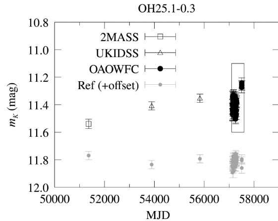
Figure 1: K-band light curve of a non-variable OH/IR star obtained by the 2MASS, UKIDSS, and OAOWFC surveys [1]. The black points are the data of OH 25.1–0.3, and the gray points are those of a reference object close to OH 25.1–0.3.
