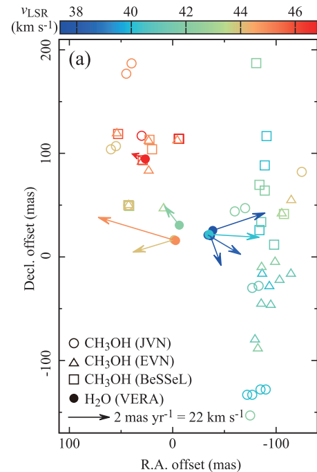
Figure 2: H 2 O maser feature distribution with internal motion (filled circles with arrows); 2 mas yr -1 corresponds to 22 km s -1 at a distance of 2.31 kpc. The open circles, triangles, and squares represent the positions of the 6.7 GHz CH 3 OH masers observed by JVN, EVN, and BeSSeL, respectively.
