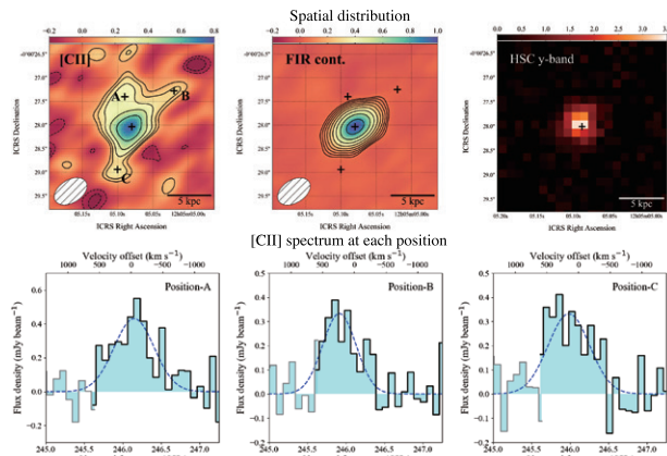
Figure 1: (Top) Spatial distributions of [CII], FIR continuum, and HSC y-band emissions of J1205–0000. The [CII] distribution is disturbed, indicating recent vigorous activities. (Bottom) [CII] spectra taken at three positions of the extended [CII] emission. The signals are significantly detected, confirming the genuine existence of that extended component.
