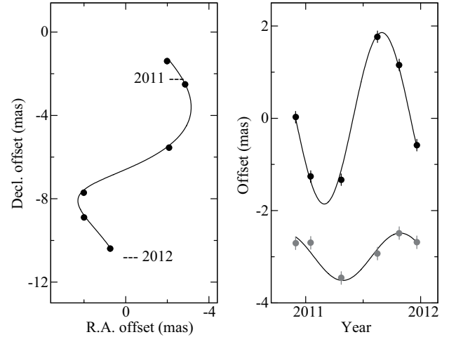
Figure 1: Parallax and proper motion of the H 2 O maser spot at in L 1482. Left panel: Positional variation on the sky. Right panel: RA (black circles) and Dec (gray circles) offset versus time. The proper motion has been removed, allowing the effects of only the parallax to be seen.
