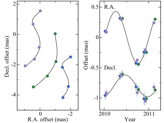
Figure 1: Parallax and proper motion fits of the maser spot at v_{\text{LSR}} = 46.4 (purple), 43.9 (green), and 42.0 km s -1 (blue). Left panel: Positional variation on the sky. Right panel: Positional variation versus time. The proper motion has been removed, allowing the effects of only the parallax to be seen.
