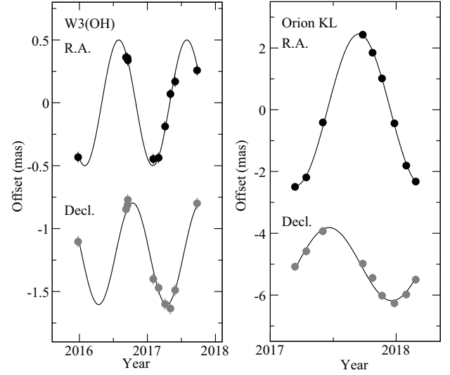
Figure 1: Parallaxes of W3(OH) (left) and Orion KL (right) obtained using VEDA. The black and gray circles show the R.A. and Decl. offsets, respectively. The solid lines show the best-fit parallaxes of 0.527 \pm 0.016 mas for W3OH and 2.459 \pm 0.029 mas for Orion KL.
