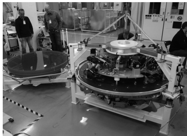
Figure 2: TIO inspected Japan's mirror polishing and measurement processes. In December 2020, the first quality review was conducted for a segment mirror that underwent the aspherical polishing process. This mirror, which was one of the mirrors polished in FY 2019, successfully passed the review, and will be cut into a hexagonal shape in the next step.
