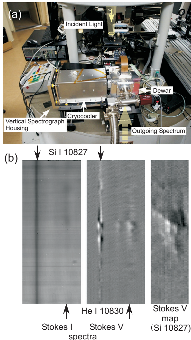
Figure 1: (a) Experimental setup of the H2RG camera system deployed on the top-table of the vertical spectrograph of the Domeless Solar Telescope. (b) Polarimetry data obtained from an experimental observation on 2018 November 20. In the sample Stokes I and V / I spectra including the Si I 1082.7 nm and He I 1083.0 nm lines, the polarization signals produced by the magnetic field can be found. We composed a Stokes V / I map, taken in the blue wing of the Si I 1082.7 nm line, from the data acquired at 26 slit positions. The map covers a field of view of 3'.7 (along the slit) × 52" including a plage region NOAA 12727. The solar north is rotated counterclockwise from the top by 6°.
