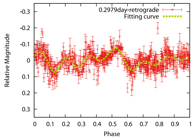
Figure 1: Lightcurve of 107P.
