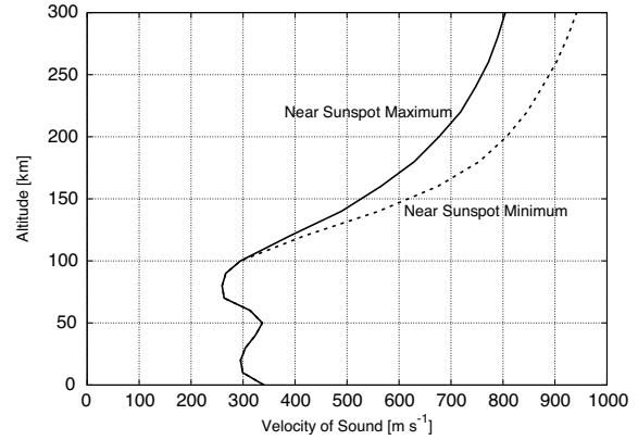
図9 Altitude with speed of sound for neutral gas 25)
